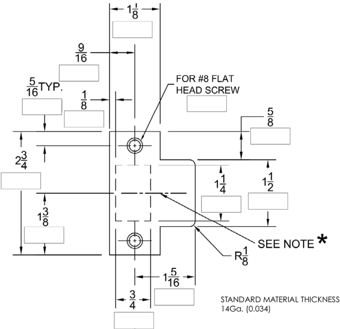
Custom "T" Strike
