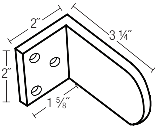
3550.3 1/4 Extended Gate Stop Price: ..... $108.00
