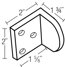
3550.1 3/4 Standard Gate Stop Price: ..... $69.00
