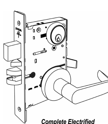
Complete Electrified Mortise Lock with SS Trim
