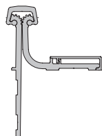
Half Surface Wide Throw
