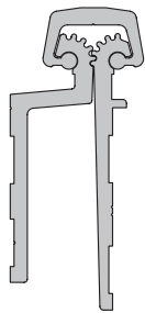
Full Mortise Short Leaf Inset Safety Hinge
