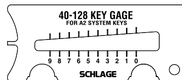
40-128 SFIC Key gage
