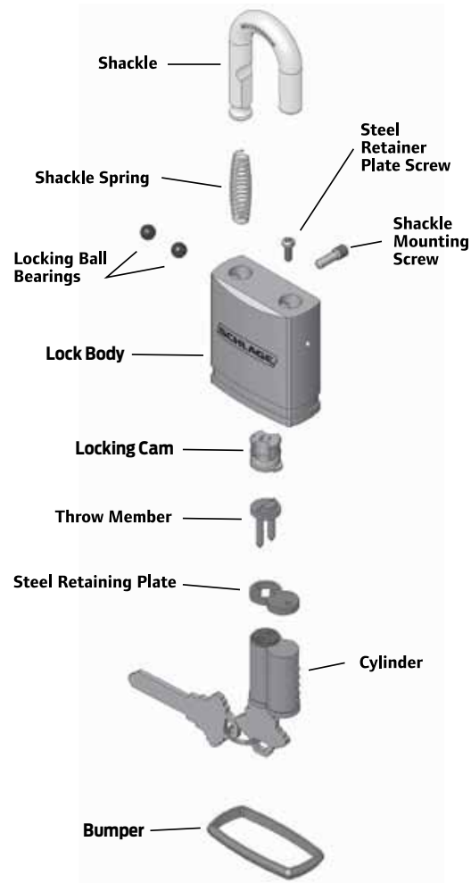
Small Format Interchangeable Core
