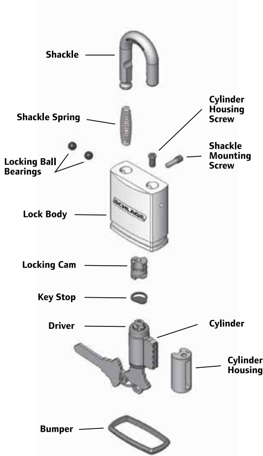
Conventional Key-in-Lever
